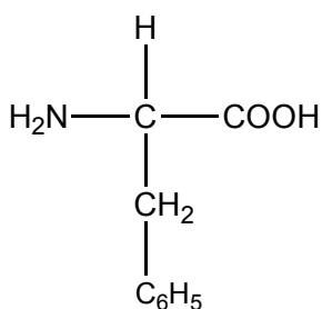
phenylalanine
